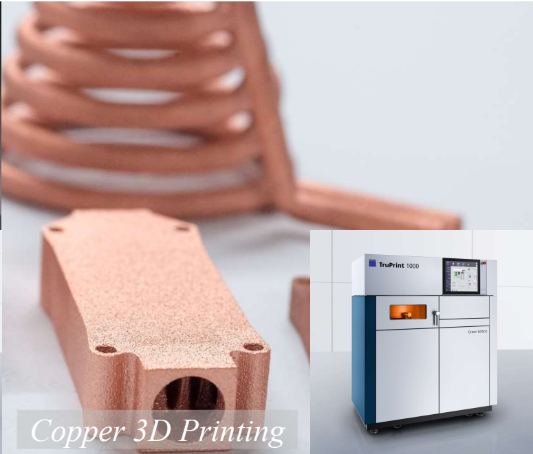
TruPrint 1000 Green Edition
