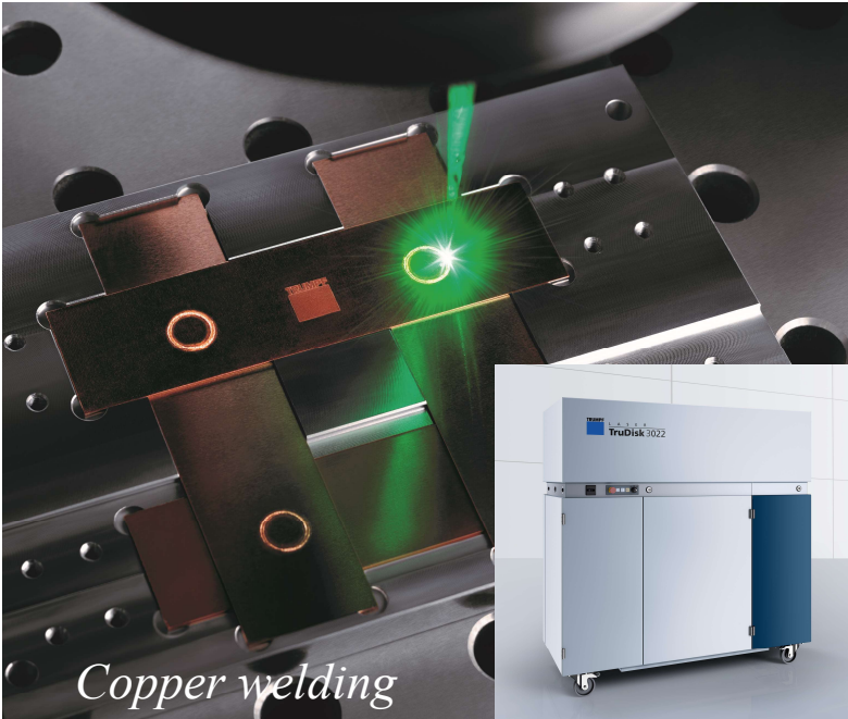
TruDisk 3022 with BrightLine Weld
