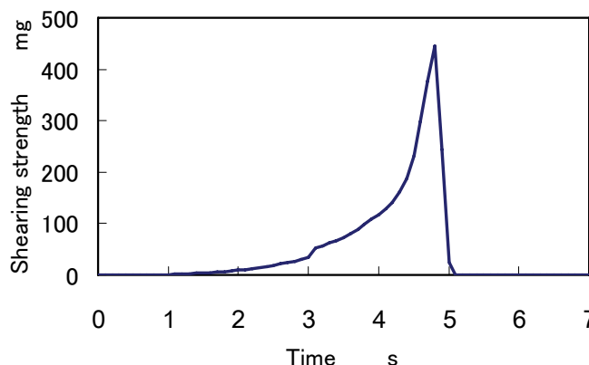
Fig. 6 Single shearing test result.
