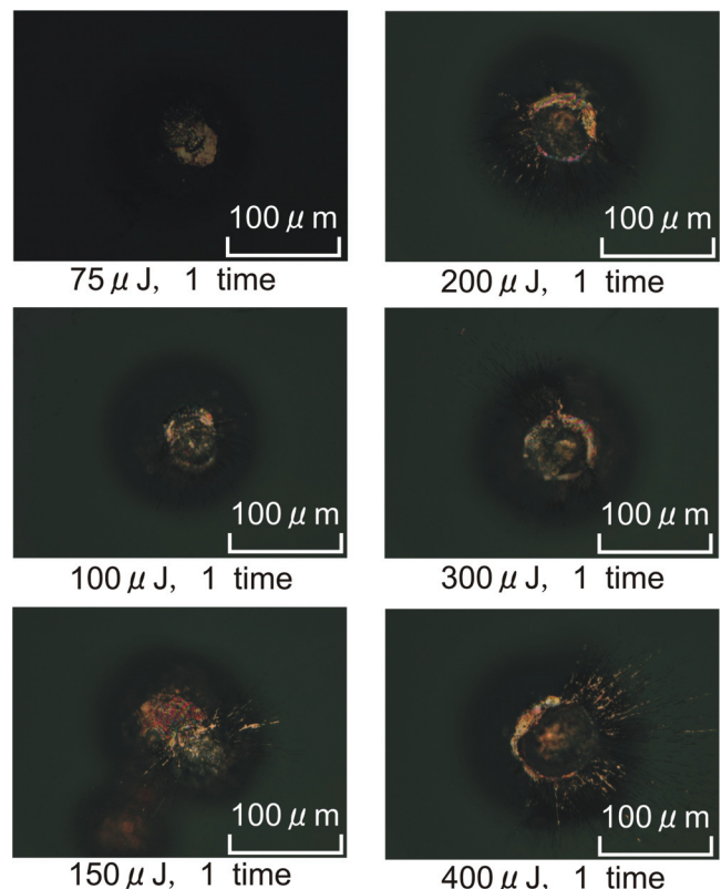
Fig. 3 Appearance of the bonding area through the cover glass for a single irradiation at various pulse energies.
