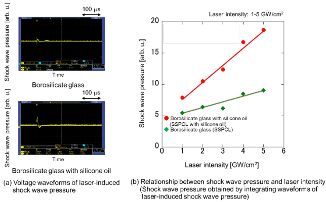
Fig. 4 Laser-induced shock wave pressure measured by PVDF gauge.
