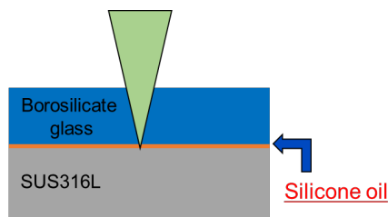
Fig. 2 To improve the impedance mismatch, silicone oil was used to reduce the acoustic impedance mismatch between the sample and the glass.
