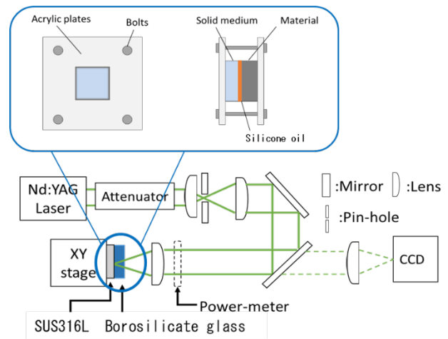
Fig. 5 Experimental setup for laser peening.
