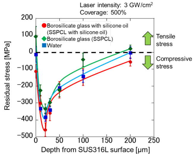
Fig. 7 Residual stress in laser-peened samples with various plasma confinement layers.
