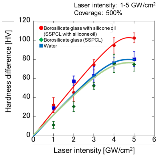
Fig. 6 Surface hardness of laser-peened samples with various plasma confinement layers.
