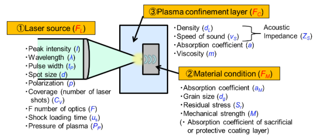
Fig. 1 Parameters for laser peening.
