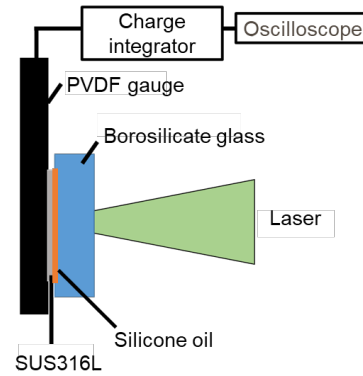
Fig. 3 Experimental setup for measurement of laser-induced shock wave pressure by PVDF gauge.
