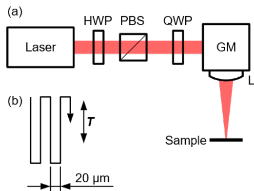
Fig. 1 (a) Schematic representation of the optical setup. HWP: half-wave plate; PBS: polarizing beam splitter; QWP: quarter-wave plate; GM: galvanometer scanner; L: lens. (b) Irradiation trajectory pattern. T indicates the orientation of the long side of the zig-zag pattern.
