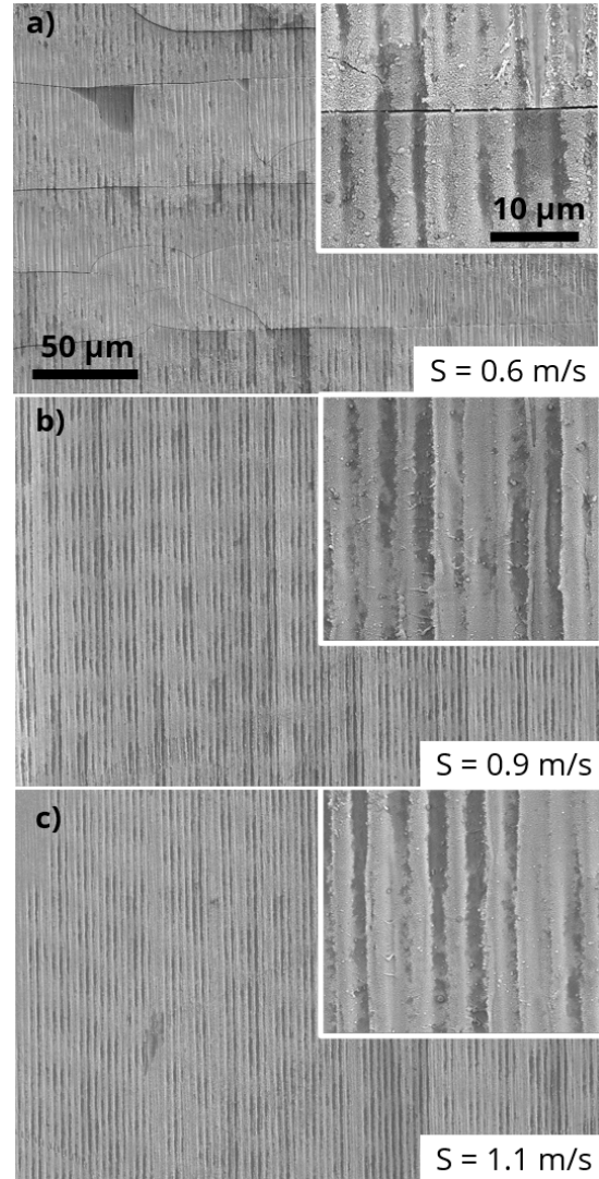
Fig. 2 Selected SEM images of soda-lime glass structured using DLIP with a single pass at a scanner speed S of a) 0.6 m/s, b) 0.9 m/s, and c) 1.1 m/s. All samples present a single-scale texture featuring a line-like pattern.
