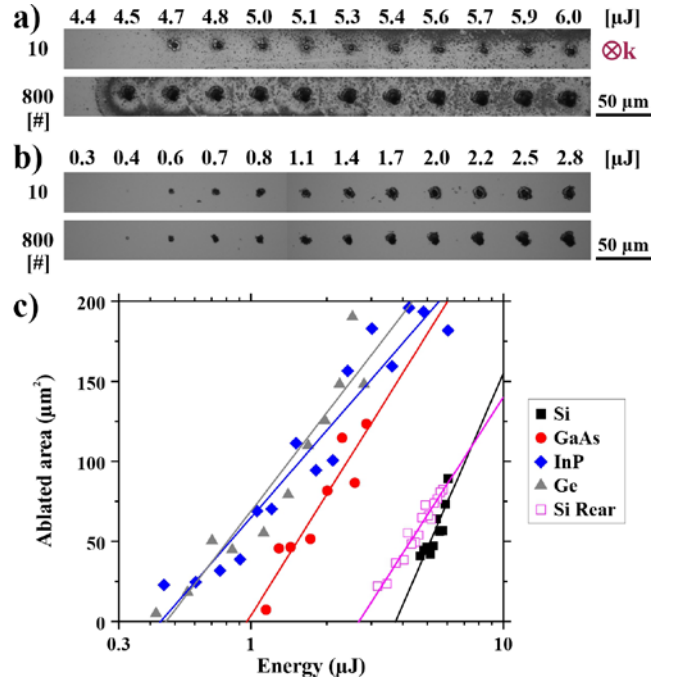
Fig. 5 Optical microscopy images of ablated spots on the surface of a) Si and b) Ge. c) Measured area of the ablation spots performed on Si, GaAs, InP, and Ge at different pulse energies and 10 pulses. Lines correspond to a fit accounting for a thresholding of a Gaussian energy distribution (Table 1). Adapted from [19], with permission.
