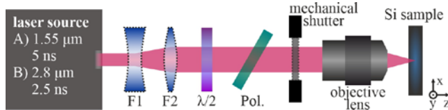
Fig. 1 Schematic representation of the experimental setup comprising the ns laser source, beam expander (F1, F2), \lambda/2 , polarizer, mechanical shutter and focusing objective lens, and semiconductor sample on xyz motorized stages.
