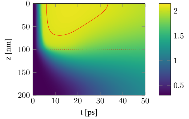
(d) Lattice temperature T_l for a peak fluence of F = 0.86 \text{ J/cm}^2 . The maximum reached temperature is T_{l,\max} = 2104.9 \text{ K} .
