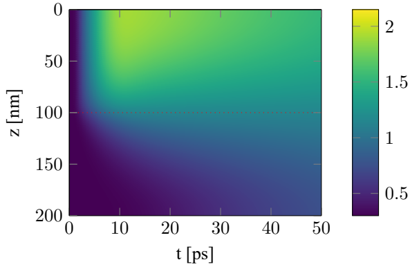
(a) Lattice temperature T_l for a peak fluence of F = 0.22 \text{ J/cm}^2 . The maximum reached temperature is T_{l,\max} = 1908.6 \text{ K} .
