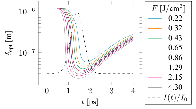
Fig. 4 Computation of the temporal evolution of the optical penetration depth \delta_{\text{opt}} = \delta_{\text{opt}}(n_e(t)) for laser pulses with different peak fluences, ranging from 0.22 J/cm 2 to 4.3 J/cm 2 .
