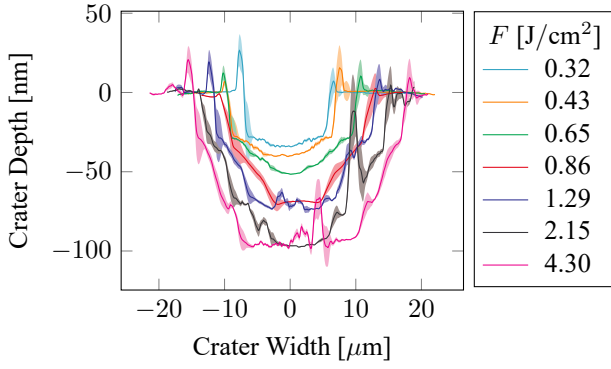
Fig. 2 Measured single pulse ablation craters with an AFM for peak fluences in ranging from 0.32 J/cm 2 to 4.3 J/cm 2 . Three depth plateaus are revealed: first plateau at 30 nm, second plateau at 70 nm and a third plateau at 100 nm, which is equal to the ITO layer thickness.
