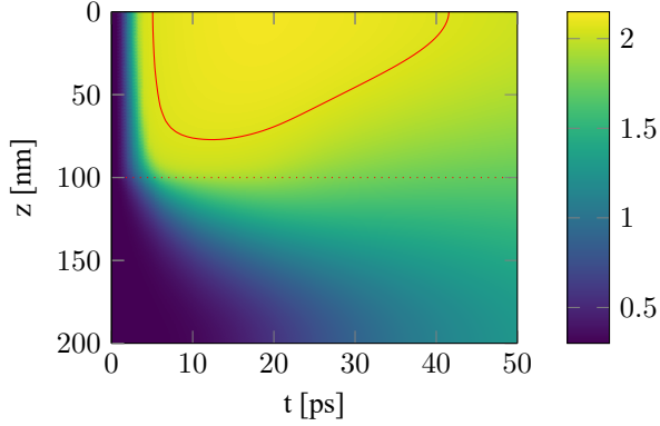
(e) Lattice temperature T_l for a peak fluence of F = 1.29 \text{ J/cm}^2 . The maximum reached temperature is T_{l,\max} = 2132.5 \text{ K} .
