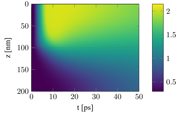
(b) Lattice temperature T_l for a peak fluence of F = 0.32 \text{ J/cm}^2 . The maximum reached temperature is T_{l,\max} = 2056.6 \text{ K} .
