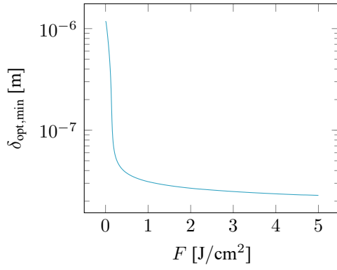
Fig. 6 Minimum optical penetration depth of the ITO film for different peak fluences.
