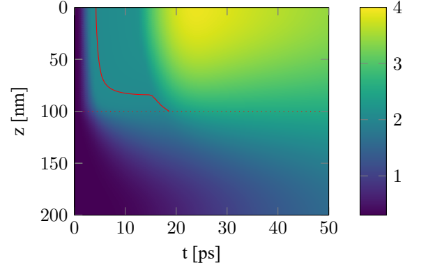
(f) Lattice temperature T_l for a peak fluence of F = 2.15 \text{ J/cm}^2 . The maximum reached temperature is T_{l,\max} = 3926.4 \text{ K} . Please note the different colorbar.
