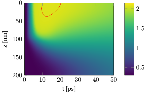
(c) Lattice temperature T_l for a peak fluence of F = 0.43 \text{ J/cm}^2 . The maximum reached temperature is T_{l,\max} = 2101.6 \text{ K} .
