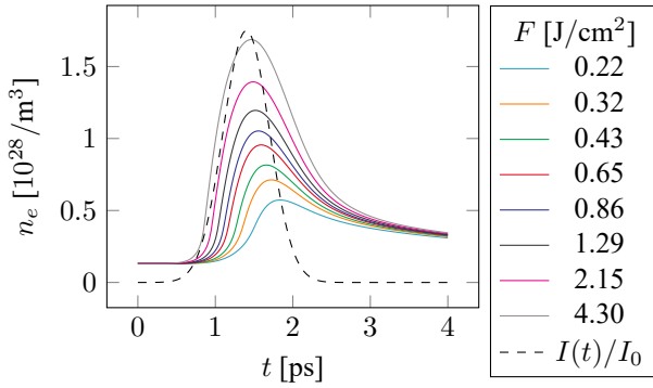
Fig. 3 Temporal evolution of the free electron density n_e at the material surface ( z = 0 ) for different peak fluences, ranging from 0.22 J/cm 2 to 4.3 J/cm 2 .
