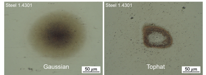
Fig. 10 Patterned areas on a steel plate 1.4301 using the superimposed gaussian and tophat beam profile. The spots are patterned using 3 pulses at a pulse energy of 29.7 µJ. The fluence per pulse for gaussian spot is 83 mJcm -2 and 636 mJcm -2 for the tophat spot.
