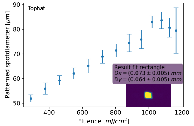
Fig. 13 Patterned spot diameter in y-direction and fluence per pulse for the tophat spot.
