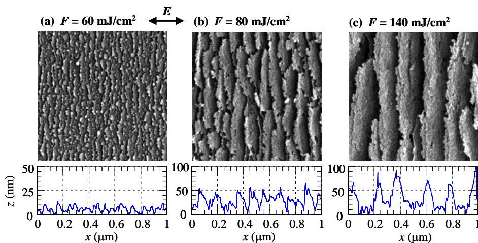
Fig. 4 SEM images and their lateral ( x - z ) scans of the DLC surface irradiated with N = 1000 of p -polarized laser pulses at (a) F = 60 \text{ mJ/cm}^2 , (b) F = 80 \text{ mJ/cm}^2 , and (c) F = 140 \text{ mJ/cm}^2 for \theta = 60^\circ . The image area, the scan direction, and the incident direction of laser pulses are the same as in Fig. 1.
