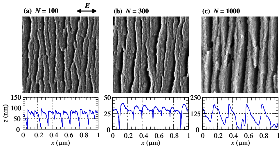
Fig. 3 SEM images and their lateral ( x - z ) scans of the DLC surface irradiated with (a) N = 100 , (b) N = 300 , and (c) N = 1000 of p -polarized laser pulses at F = 100 \text{ mJ/cm}^2 and \theta = 40^\circ . The image area, the scan direction, and the incident direction of laser pulses are the same as in Fig.1.
