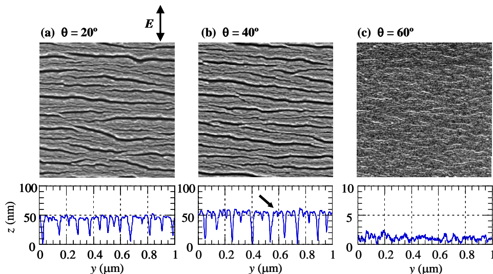
Fig. 2 SEM images and their vertical ( y - z ) scans of the DLC surface irradiated at (a) \theta = 20^\circ , (b) \theta = 40^\circ and (c) \theta = 60^\circ with N = 100 of s -polarized laser pulses at F = 120 \text{ mJ/cm}^2 . The image is for the central area of 1 \times 1 \mu\text{m}^2 on the focal spot. The scan is along the polarization ( y ) direction denoted by the arrow E , and the ordinate of z = 0 indicates the lowest z position in the observed area with the SPM. The arrow in (b) denotes the incident direction of laser pulses.
