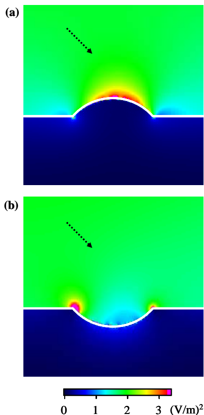
Fig. 5 Calculated field intensity distribution around (a) a hill and (b) a valley on the DLC surface irradiated with p -polarized light incident at \theta = 40^\circ . The hill and valley are assumed to have the radius of 30 nm with the height and depth of 10 nm. The arrows denote the incident direction of laser light.
