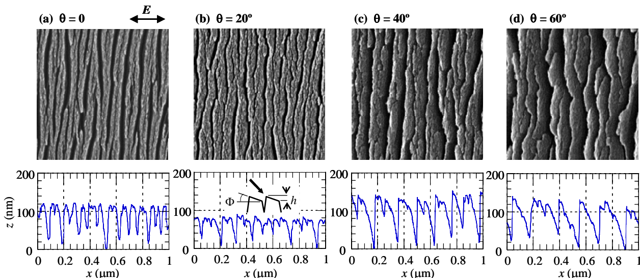
Fig. 1 SEM images and their lateral ( x - z ) scans of the DLC surface irradiated at (a) \theta = 0^\circ , (b) \theta = 20^\circ , (c) \theta = 40^\circ , and (d) \theta = 60^\circ with N = 100 of p -polarized laser pulses at F = 120 \text{ mJ/cm}^2 . The image is for the central area of 1 \times 1 \mu\text{m}^2 on the focal spot. The scan is along the polarization ( x ) direction denoted by the arrow E , and the ordinate of z = 0 indicates the lowest z position in the observed area with the SPM. The inset in (b) defines the height h and the angle \Phi of surface slope, and the arrow denotes the incident direction of laser pulses.
