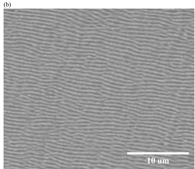
Fig. 2 SEM image of a single-point pattern irradiated at the laser fluence of 0.48 \text{ J/cm}^2 with 100 shots.
