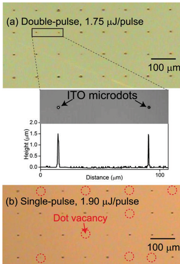
Fig.4 Confocal scanning laser microscopic images and profile of the ITO microdot arrays deposited by (a) double-pulse and (b) single-pulse LIDT, respectively. The time delay, t_d was 500 \text{ ns} . The ITO microdots with a height of 1.5 \text{ }\mu\text{m} were reproducibly arrayed by the double-pulse LIDT, whereas there were dot vacancies (red dotted circles) at a rate of approximately 30 % for the single-pulse LIDT.
