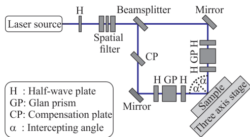
Figure 4: Schematic diagram of the two-beam interference setup
